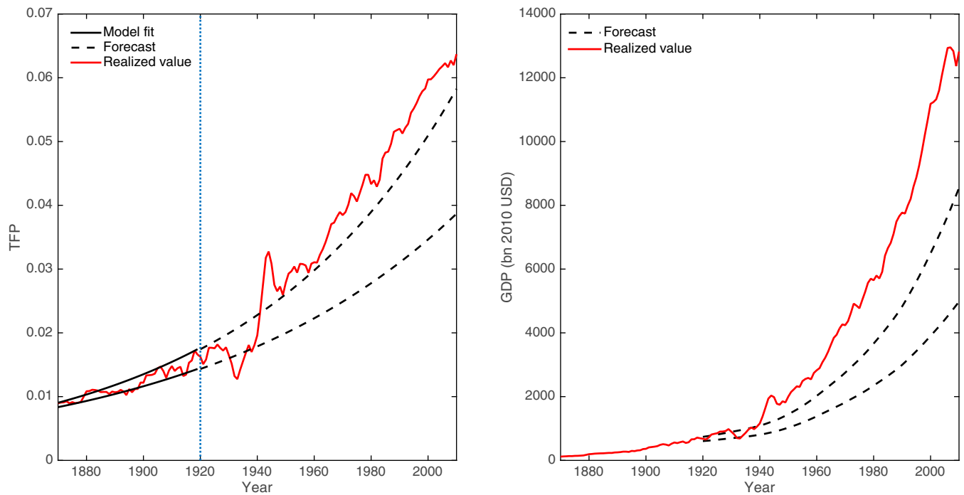
Fig. 1. Long-run forecasts of US TFP ( Left ) and economic output ( Right ) from the economic growth model used by DICE. The model was trained on the data from 1870 to 1920 and projections made in 1920. Solid red lines are realized data values. Dashed black lines are forecasts generated using model parameter values at the boundary of estimated 95% CI, and solid black lines ( Left ) show the fit of the TFP model to the data over the training window.
