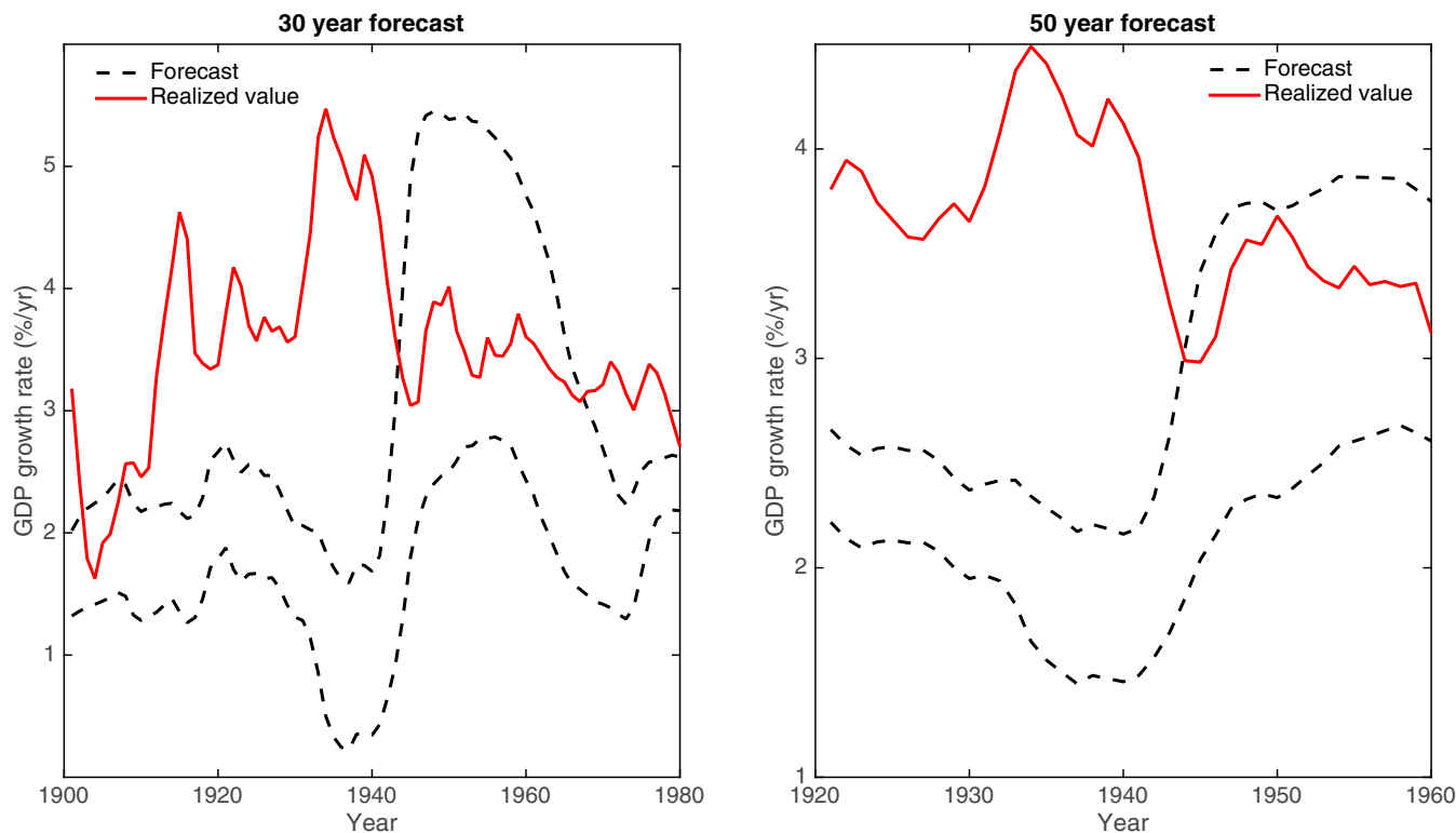
Fig. 2. Thirty-year (Left) and 50-y (Right) forecasts of US economic growth from the economic growth model used by DICE. (Left) The solid red line at date T denotes the realized compound annual growth rate over the period [T, T + 30] . The dashed black lines at date T denote the forecasted interval for the growth rate over [T, T + 30] when the model is trained on data from [T - 30, T] , using the same estimation and prediction methodology as in Fig. 1. (Right) The equivalent for 50-y training and verification windows.
